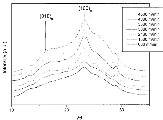
Figure 6. Equatorial wide angle X-ray diffraction profiles of as-spun fibers obtained under different spinning speeds.
