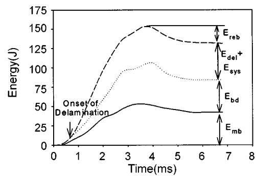
(a) QTC
