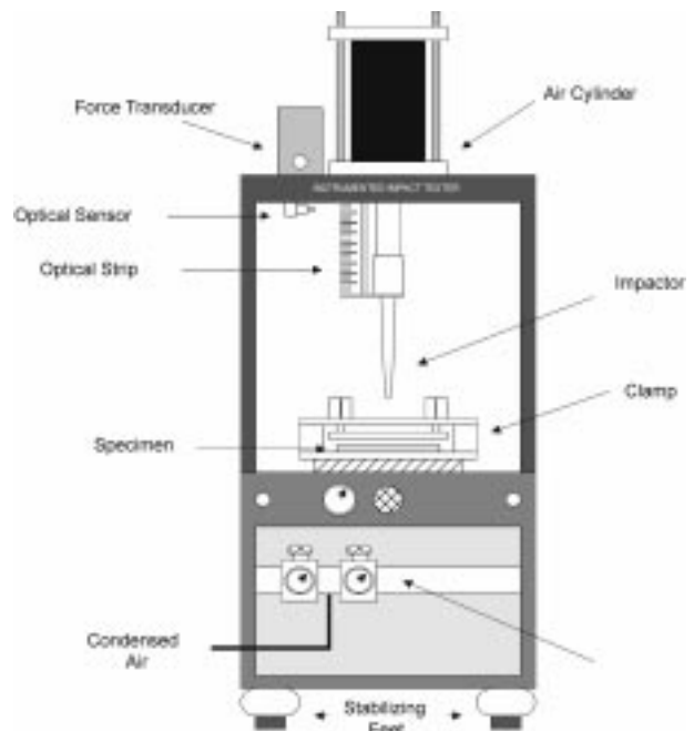
Figure 1. Instrumented impact tester.
