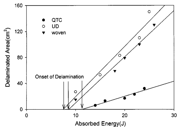
Figure 7. Impact fracture toughness.
