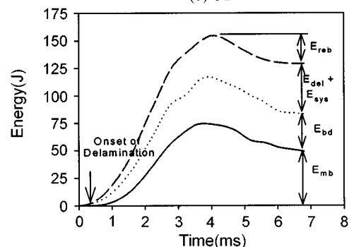
(c) Woven
